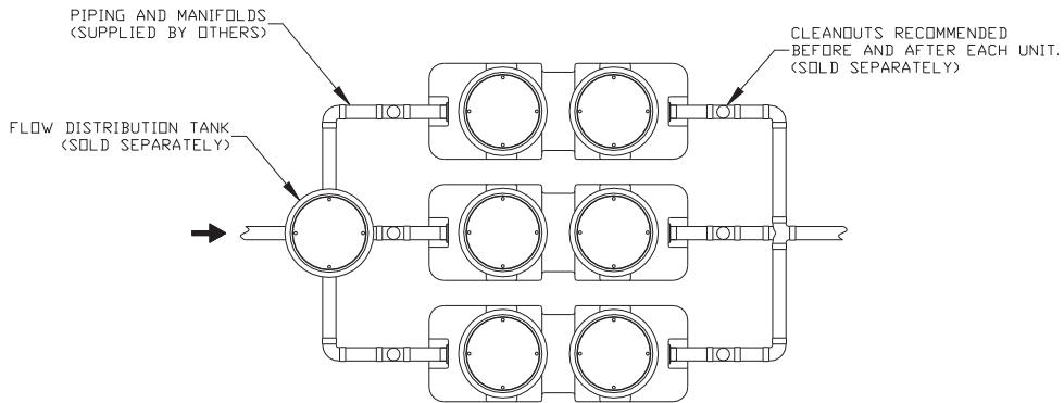
XL-MI-G-PL-1150 THREE IN PARALLEL 300 GPM, 3450 GREASE LBS. CAPACITY
