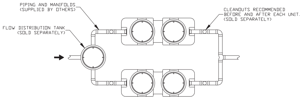
XL-MI-G-PL-1150 TWO IN PARALLEL 200 GPM, 2300 GREASE LBS. CAPACITY
