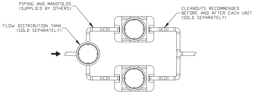
XL-MI-G-PL-750 TWO IN PARALLEL 10 GPM, 1500 GREASE LBS. CAPACITY
