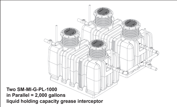
Typical piping layout for SuperMax interceptor
