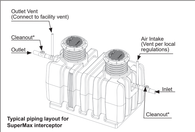
Two SM-MI-G-PL-1000 in Series = 2,000 gallons liquid holding capacity grease interceptor
