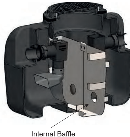
BIG-1150-IB - with internal baffle
