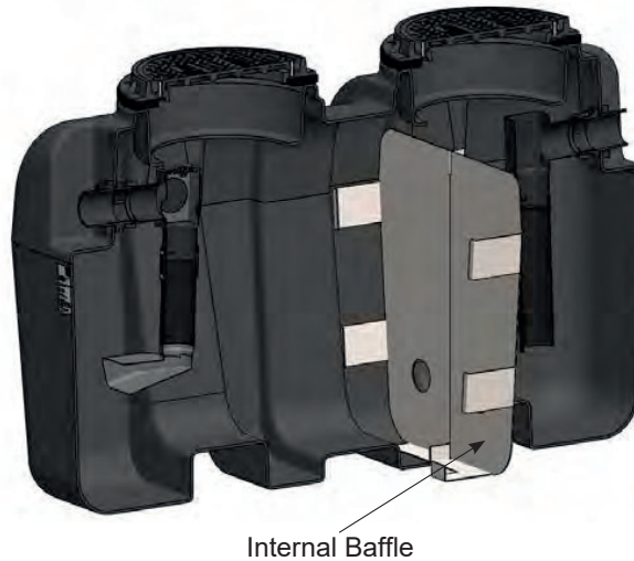
BIG-1150-IB - with internal baffle
