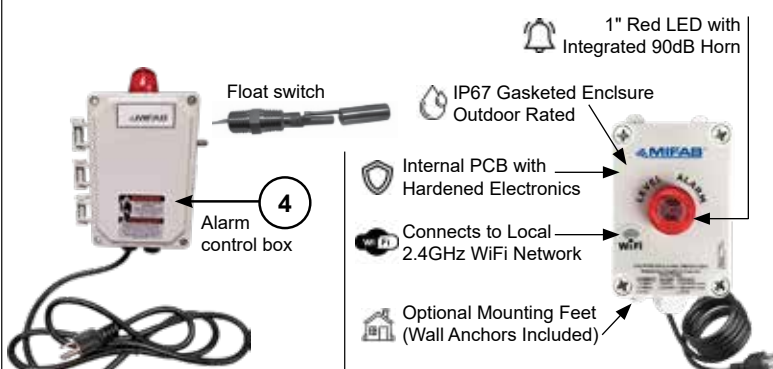
High Level Alarm Illustrated (Specify suffix -HLA)
