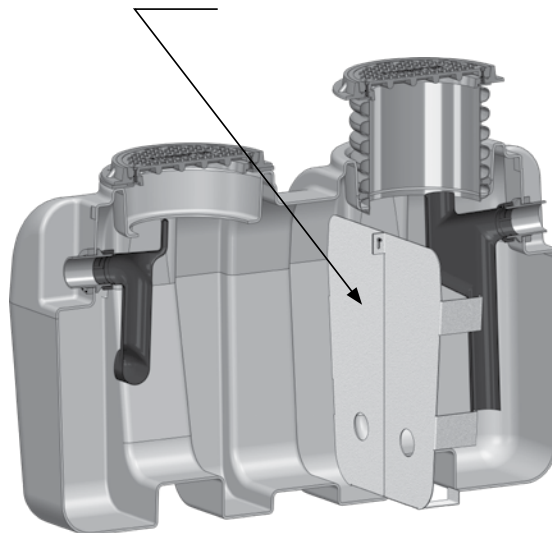
BIG-1150-IB - with internal baffle
