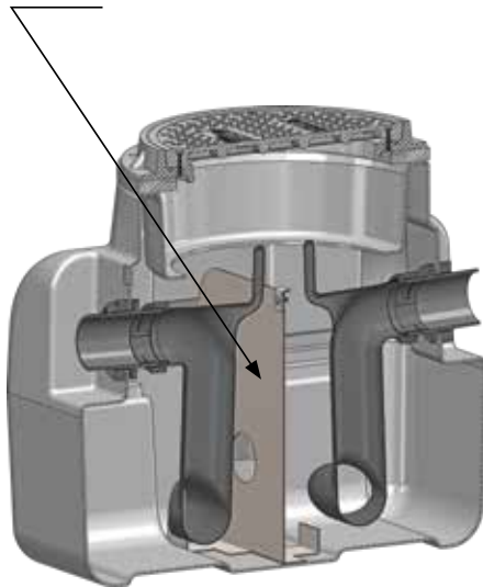
BIG-500-IB - with internal baffle
