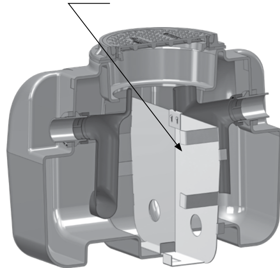
BIG-750-IB - with internal baffle
