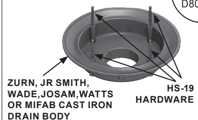
CAST IRON ROOFGUARD (MODEL #RG2016DDC)
