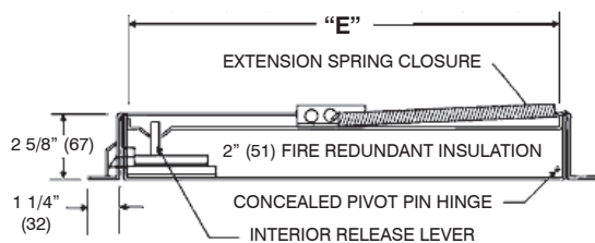
A-B Door Size C-D Overall Dimensions - Door Size - Plus 2 5/8" (67) E Wall Opening - Door Size - Plus 1/2" (13) (Allow an extra 1/4" (6) clearance for latch housing on "D" side.)
