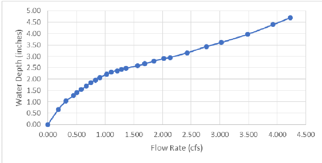
Figure 1, Rating curve
