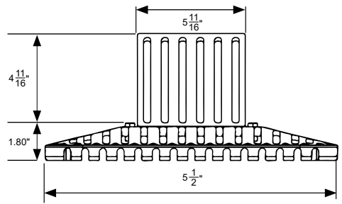
Cast iron scupper drain, less MIFAB® body for retrofit applications.
