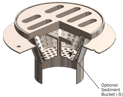
-RS Special duty slotted grate with finger holes
