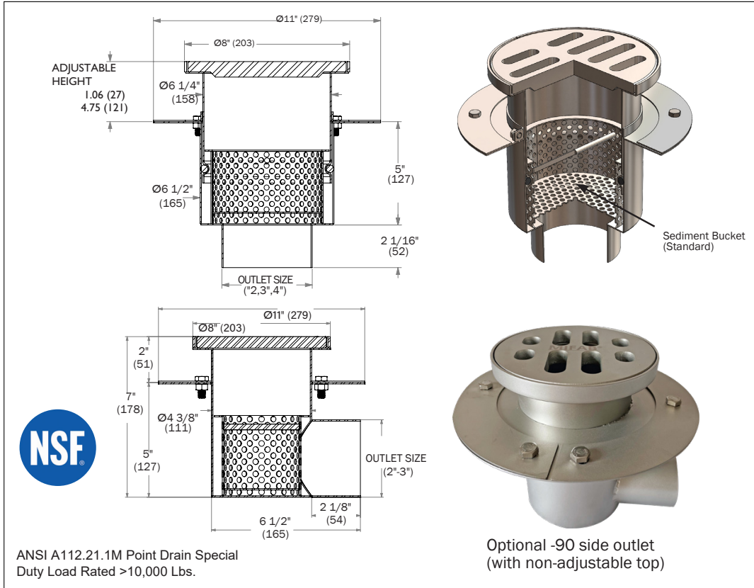
-RS Heavy duty slotted grate with finger holes
