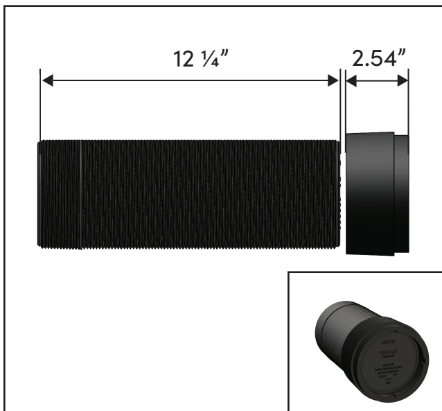
MC-10-PN12AH-31 12" Tapered Thread Nipple with Adjustable Horn at End
