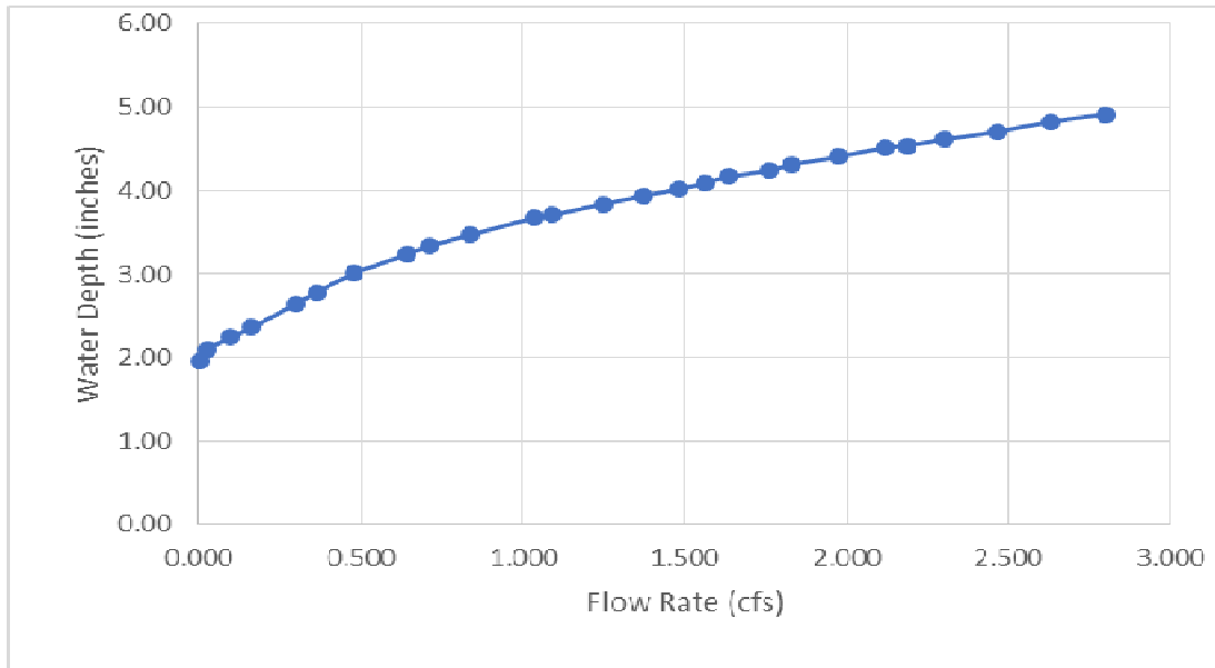
Figure 1, Rating curve
