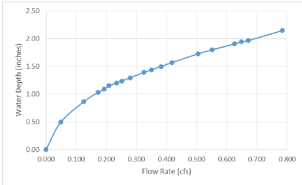
Figure 1, Rating curve
