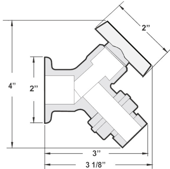
MHY-9000 Series wall faucet dimensions
