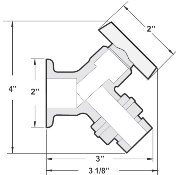
HY-9200-NPB Series wall faucet dimensions
