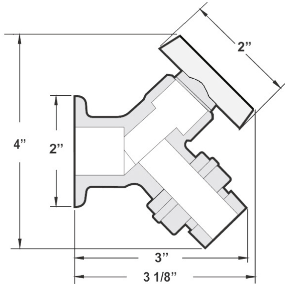
HY-9000-NPB Series wall faucet dimensions
