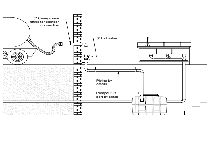
BASEMENT INSTALLTION WITH PUMPOUT KIT
