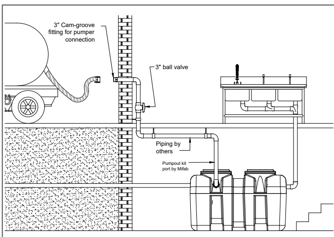
BASEMENT INSTALLATION WITH PUMPOUT KIT
