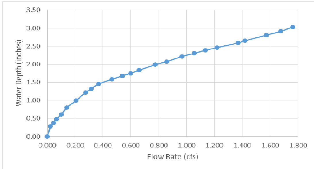
Figure 1, Rating curve
