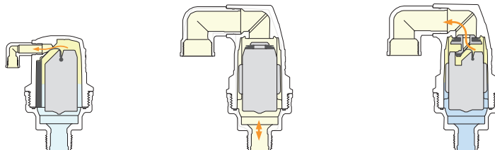
AIR RELEASE VALVE
