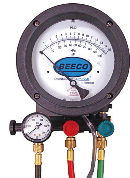
TK5-BACKFLOW-TEST (ILLUSTRATED) FOR SPEC. SHEETS GO TO www.beecobackflow.com
